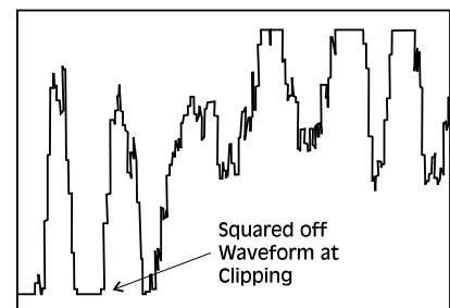
Normal Amplifier
