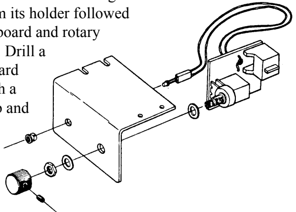
Dash Control Assembly
