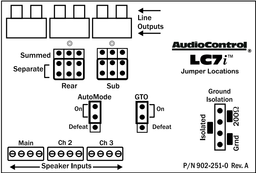
Internal Jumper Configuration
